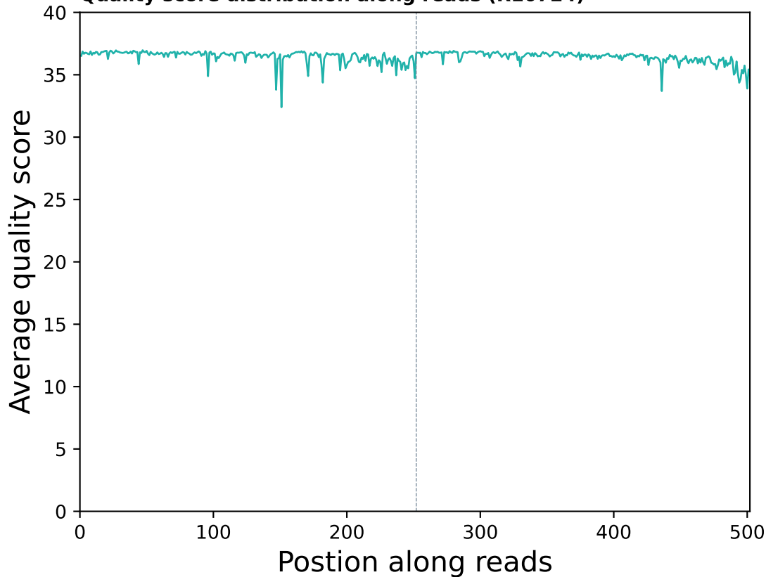
Quality score distribution along reads (R10724)
